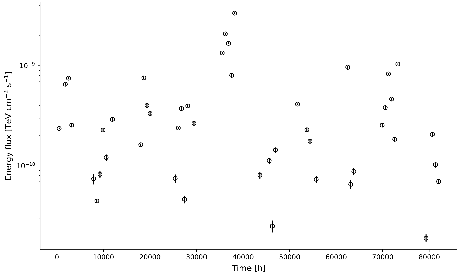
Mrk421, cadence - 2 times per month - CTAO simulation
